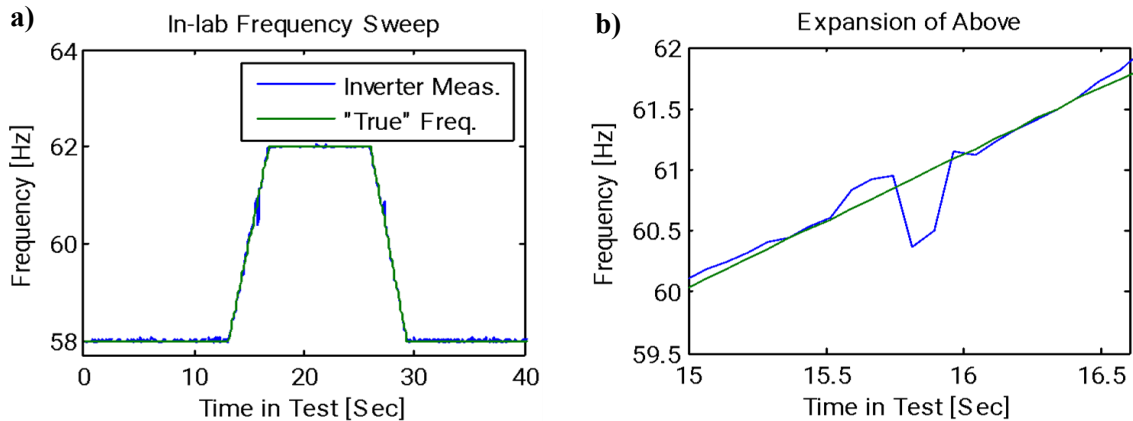
Figure 2. In-lab frequency sweep.
